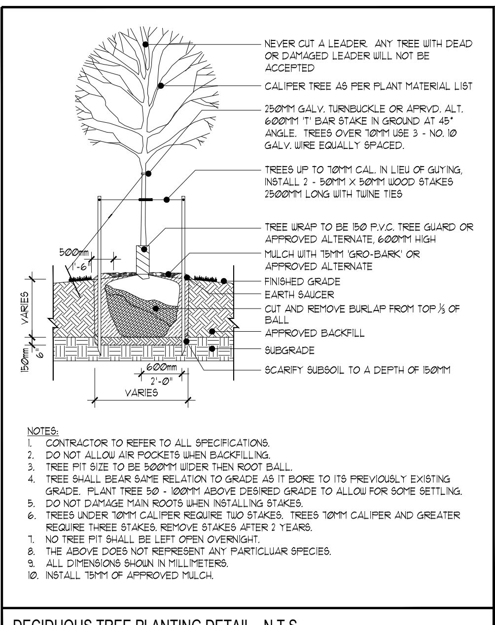
DECIDUOUS TREE PLANTING DETAIL - N.T.S.
