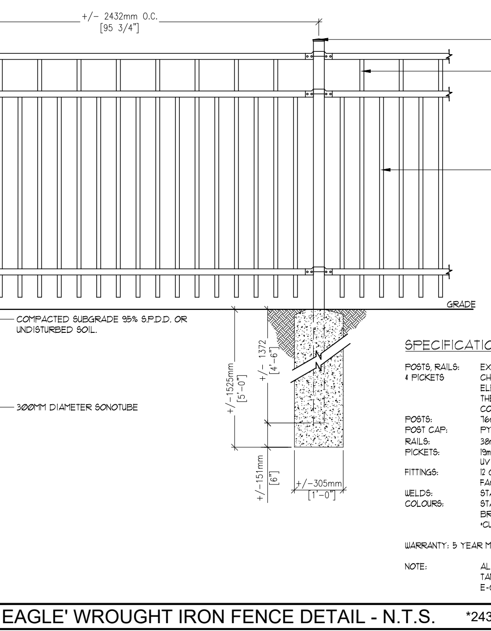
2432mm (8'-0") O.C. POST SETTING
