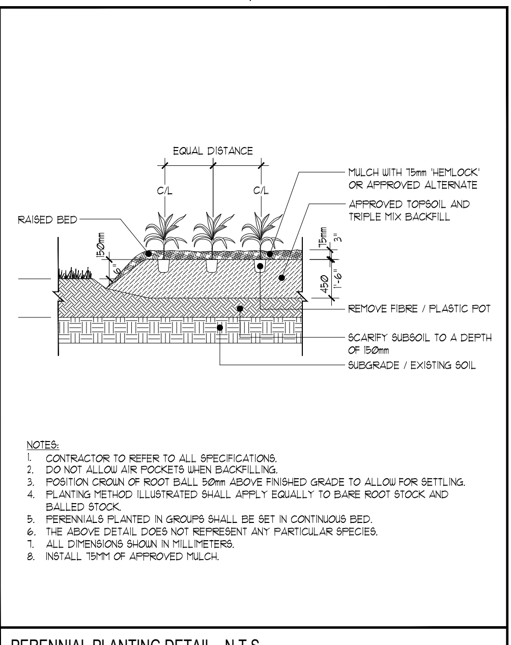
PERENNIAL PLANTING DETAIL - N.T.S.
