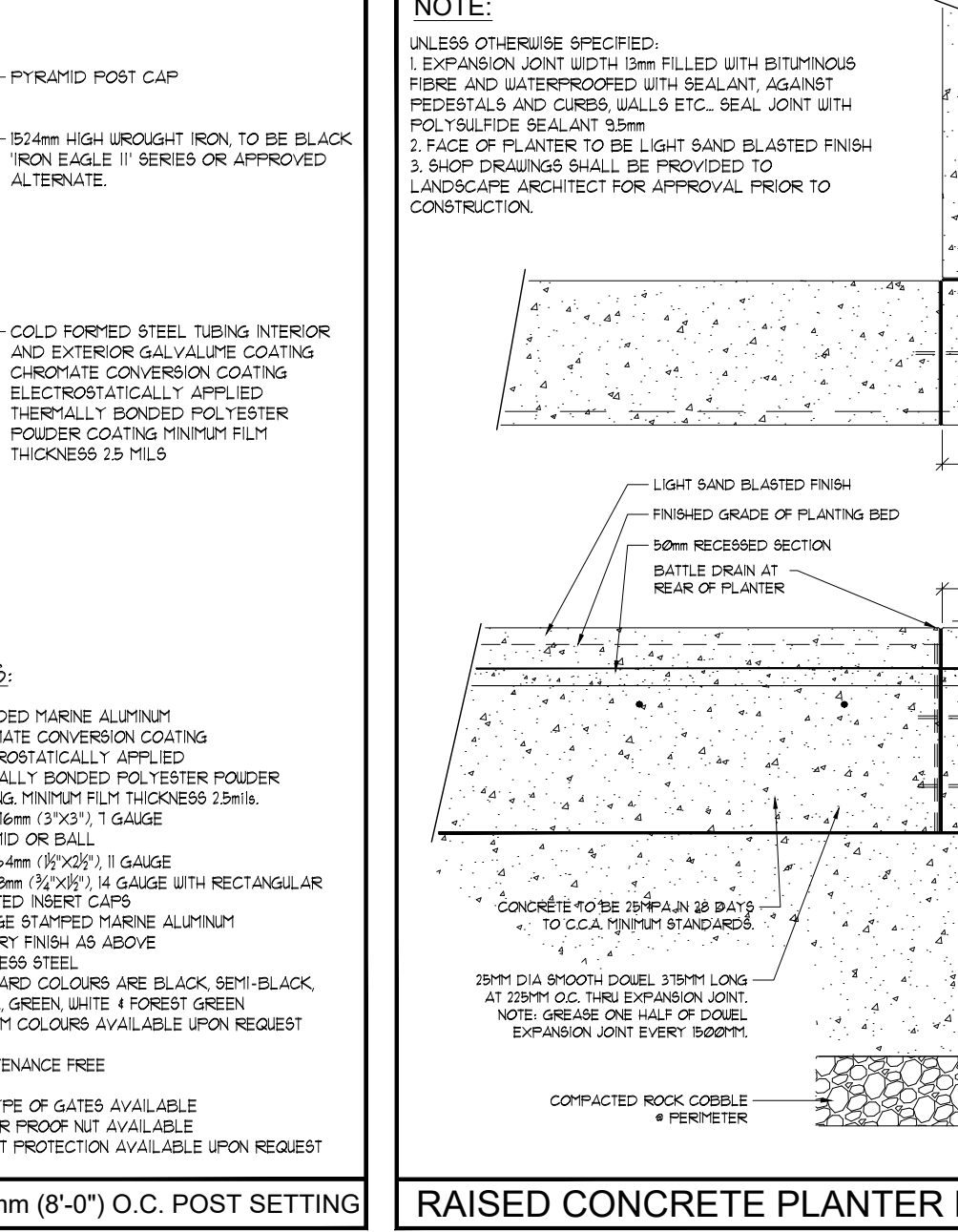
RAISED CONCRETE PLANTER DETAIL - N.T.S.
