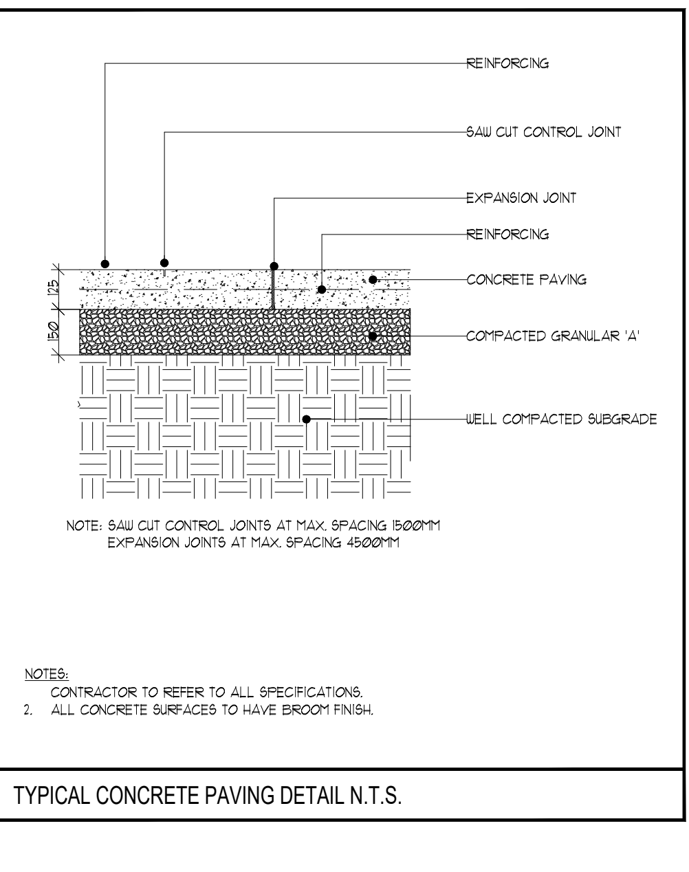
TYPICAL CONCRETE PAVING DETAIL N.T.S.
