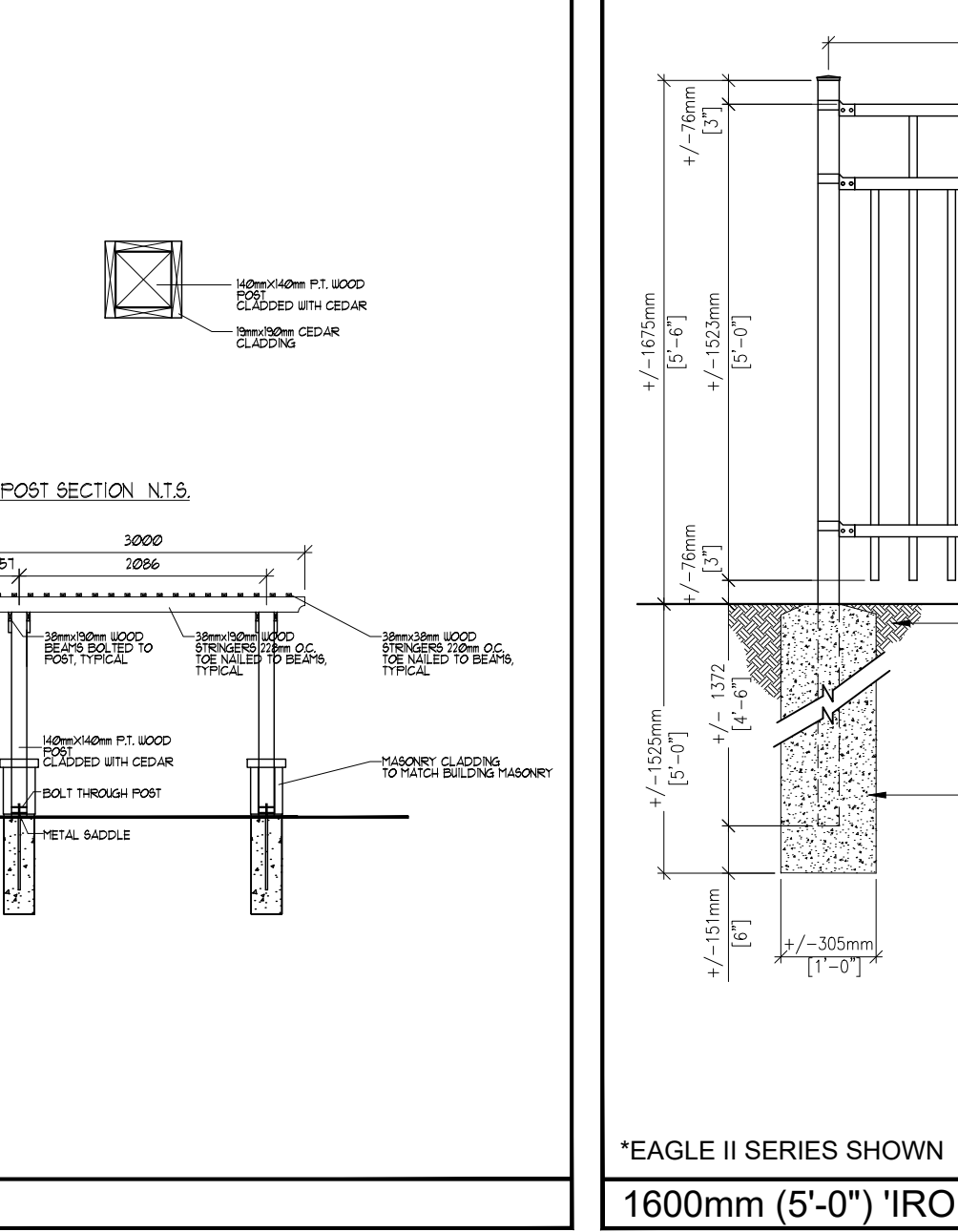
1600mm (5'-0") 'IRON EAGLE' WROUGHT IRON FENCE DETAIL - N.T.S.
