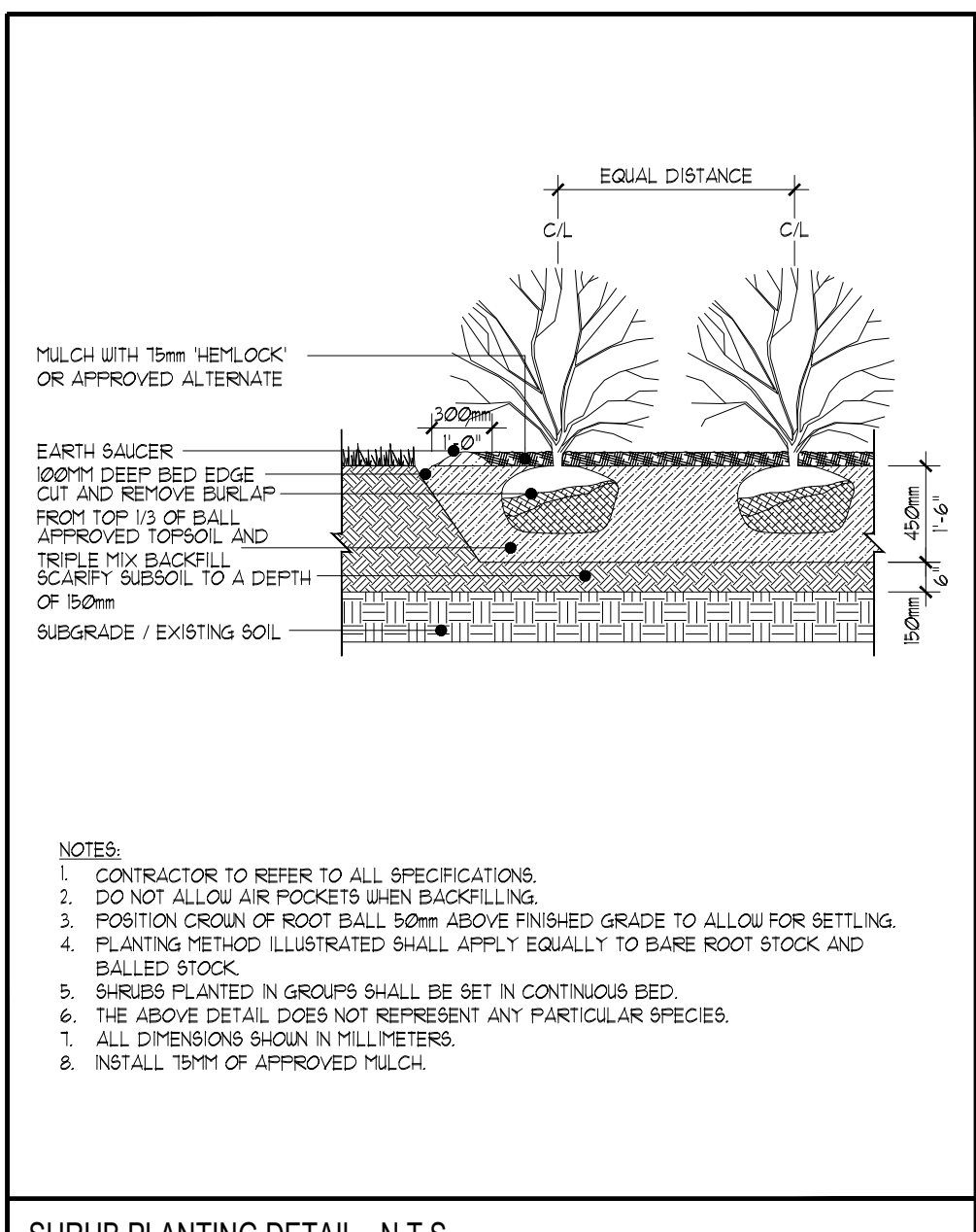
SHRUB PLANTING DETAIL - N.T.S.
