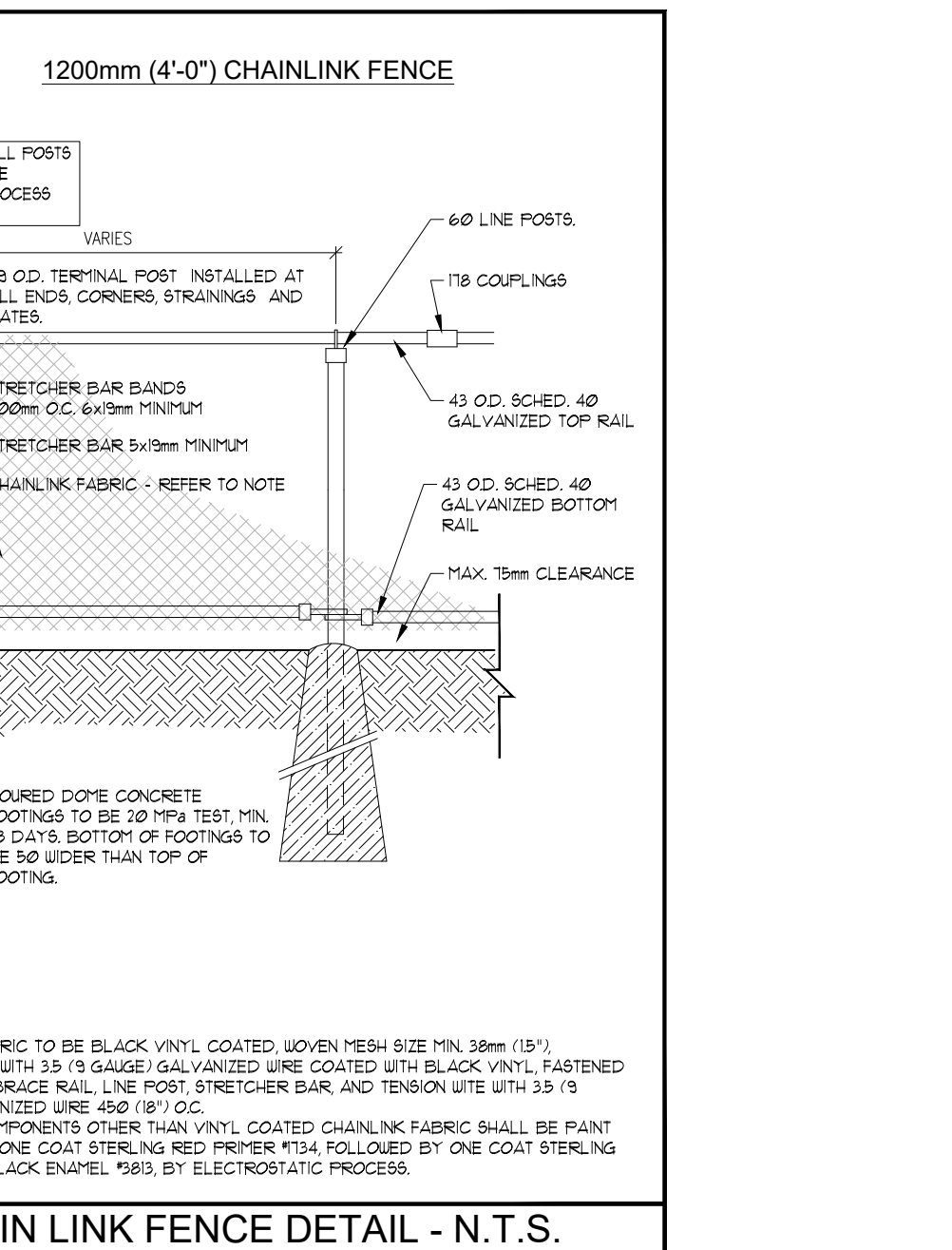
1200mm (4'-0") CHAINLINK FENCE DETAIL - N.T.S.
