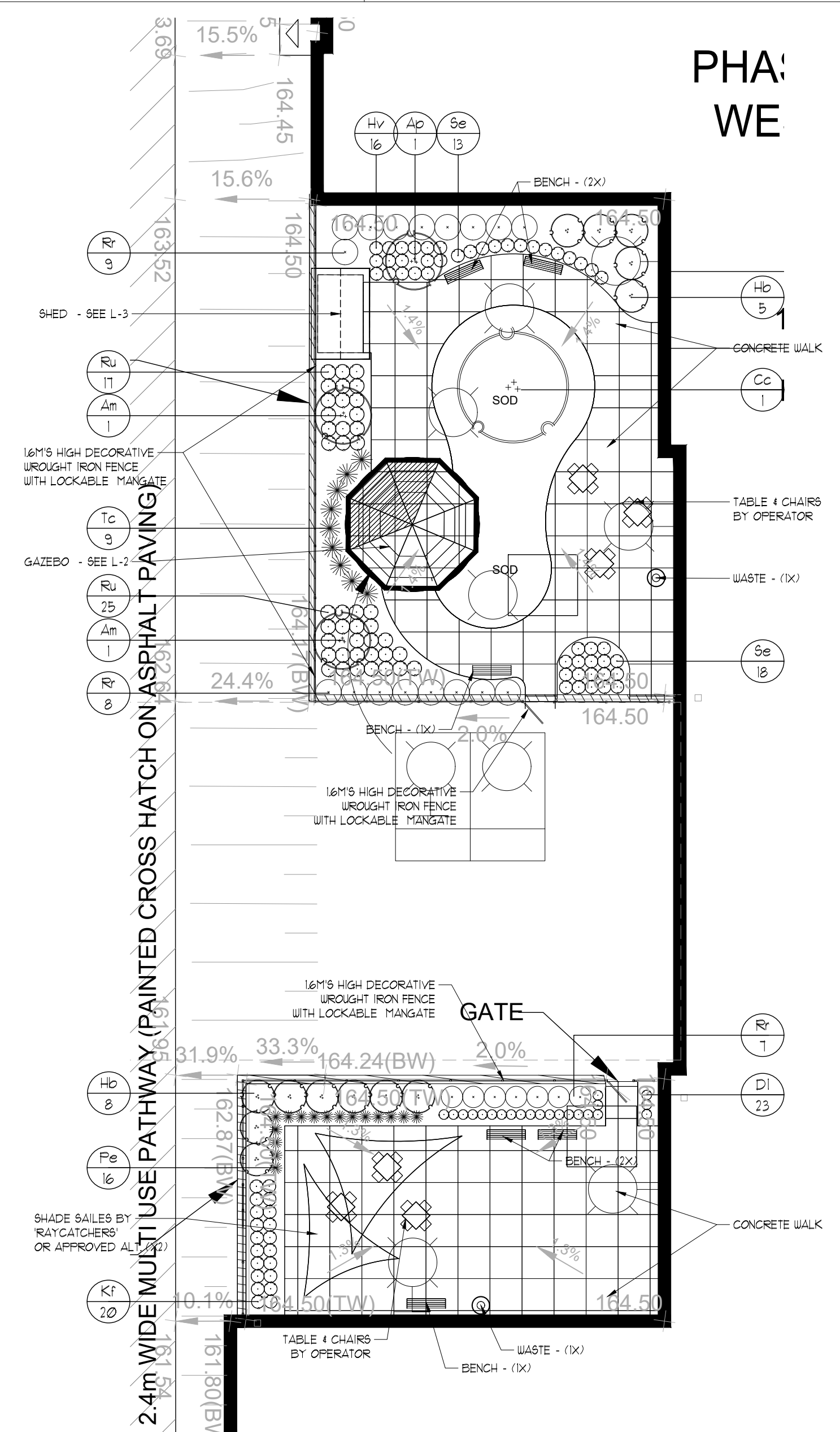
COURTYARDS 'B' & 'C' LANDSCAPE PLAN
