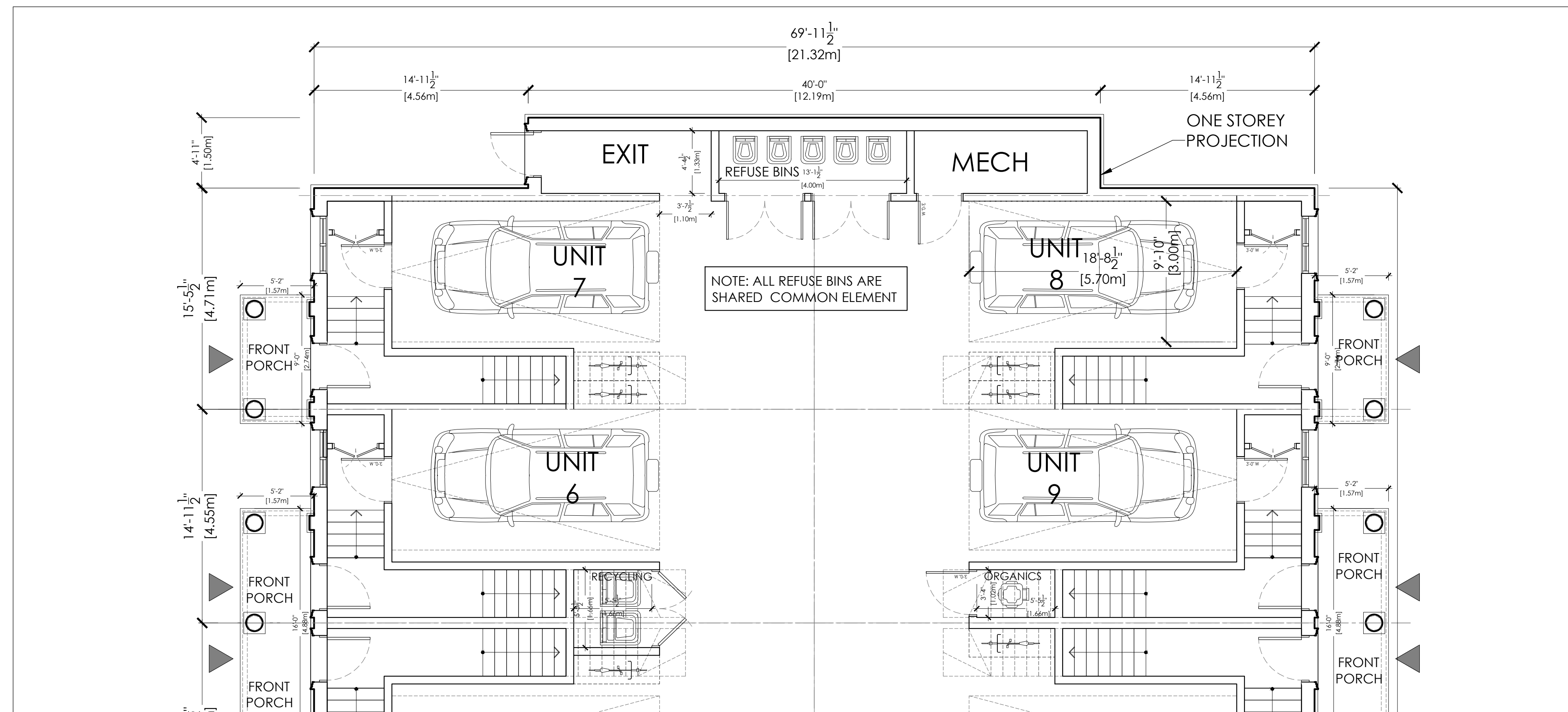
1 TYPICAL BLOCK-COMMON REFUSE ROOMS IN GARAGE SCALE: 3/16" = 1'-0"
