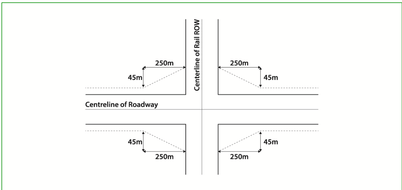
Figure 2 – Additional Land Required for a Grade Separation
